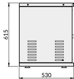
Vista lateral Vista lateral Side view
