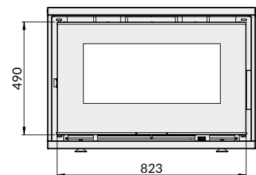
Vista frontal Vista frontal Front view
