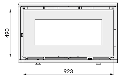
Vista frontal Vista frontal Front view
