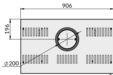
Vista topo Vista superior Top view
