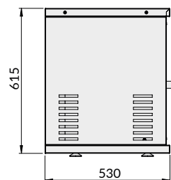
Vista lateral Vista lateral Side view
