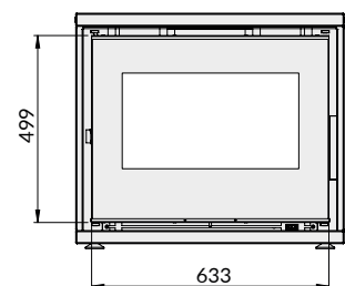
Vista frontal Vista frontal Front view
