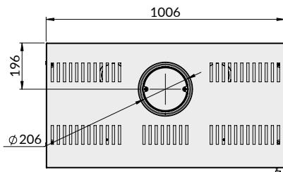
Vista topo Vista superior Top view
