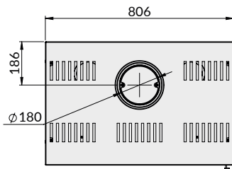
Vista topo Vista superior Top view
